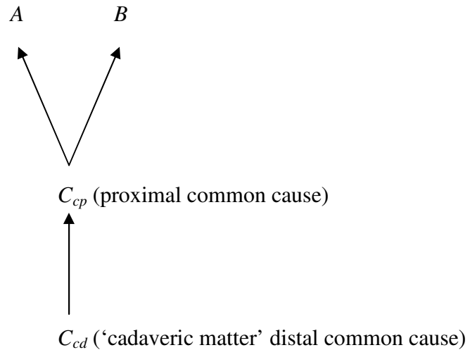
Figure 2. Proximal and distal common cause
