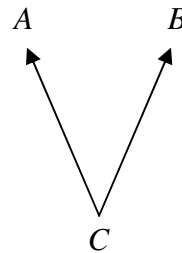
Figure 1. The conjunctive fork ACB
